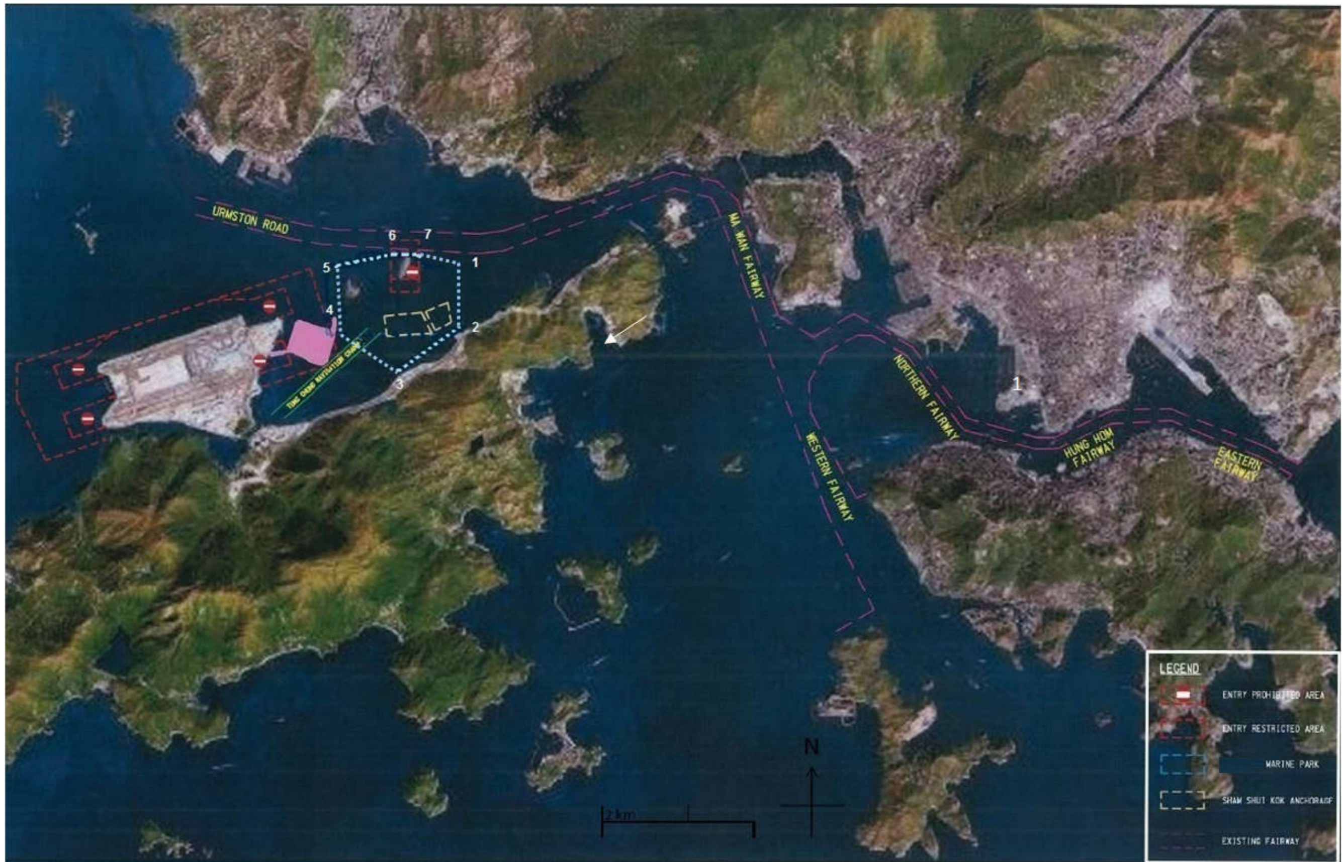
Appendix 4 Fairway Layout (Sheet 1 of 1)
