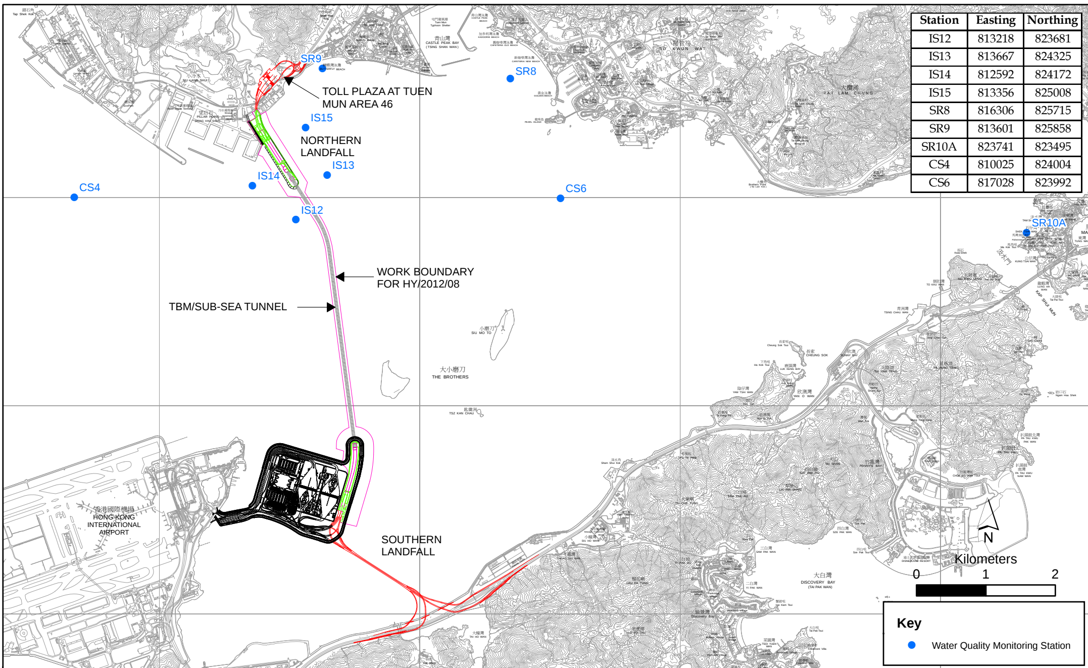
Figure 2.2 Water Quality Monitoring Station
