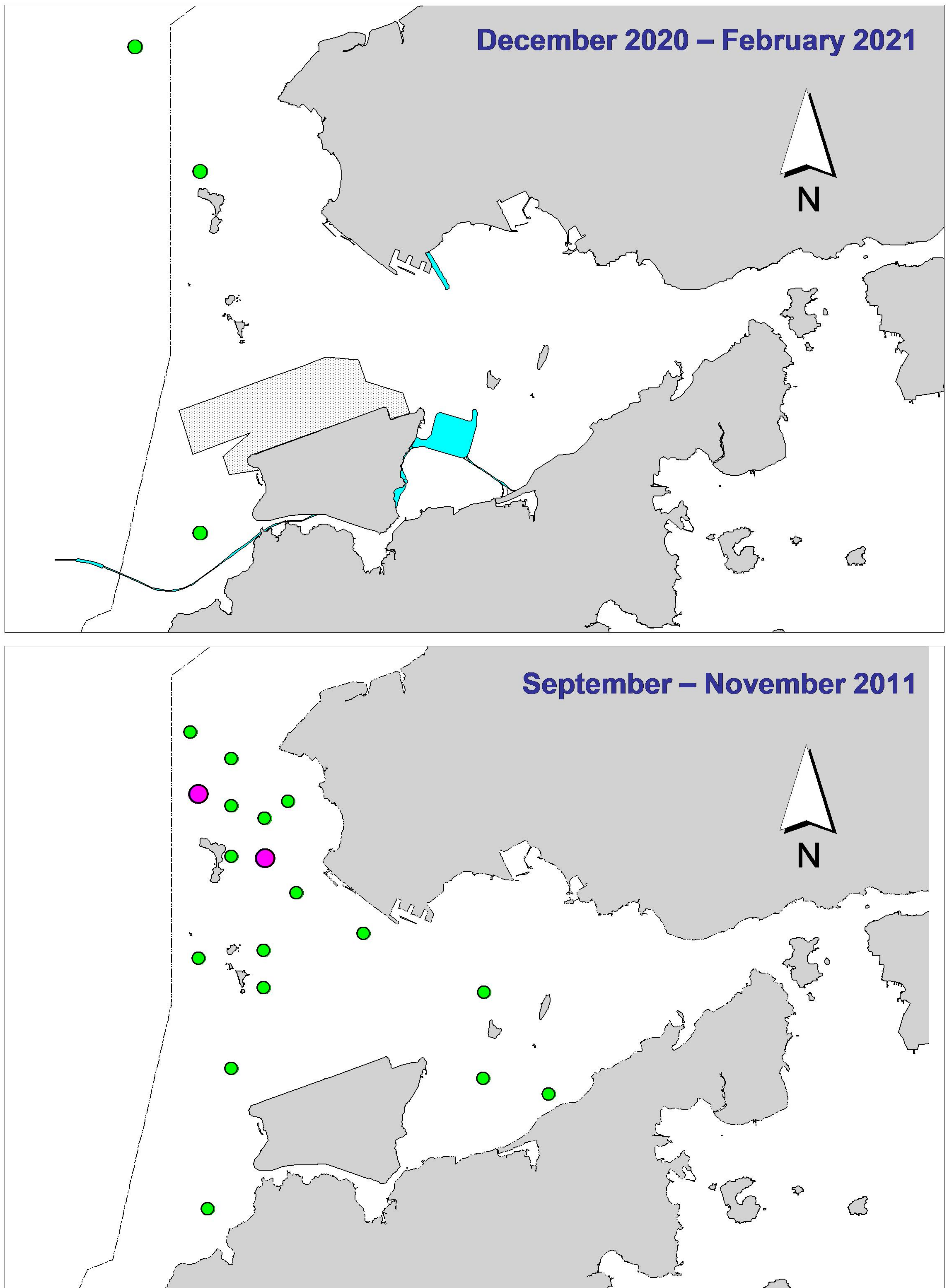
Figure 3. Distribution of Chinese white dolphins with larger group sizes during the present TMCLKL08 monitoring period (top) and baseline period in 2011 (bottom) (green dots: group sizes of 5 or more; purple dots: group sizes of 10 or more)
