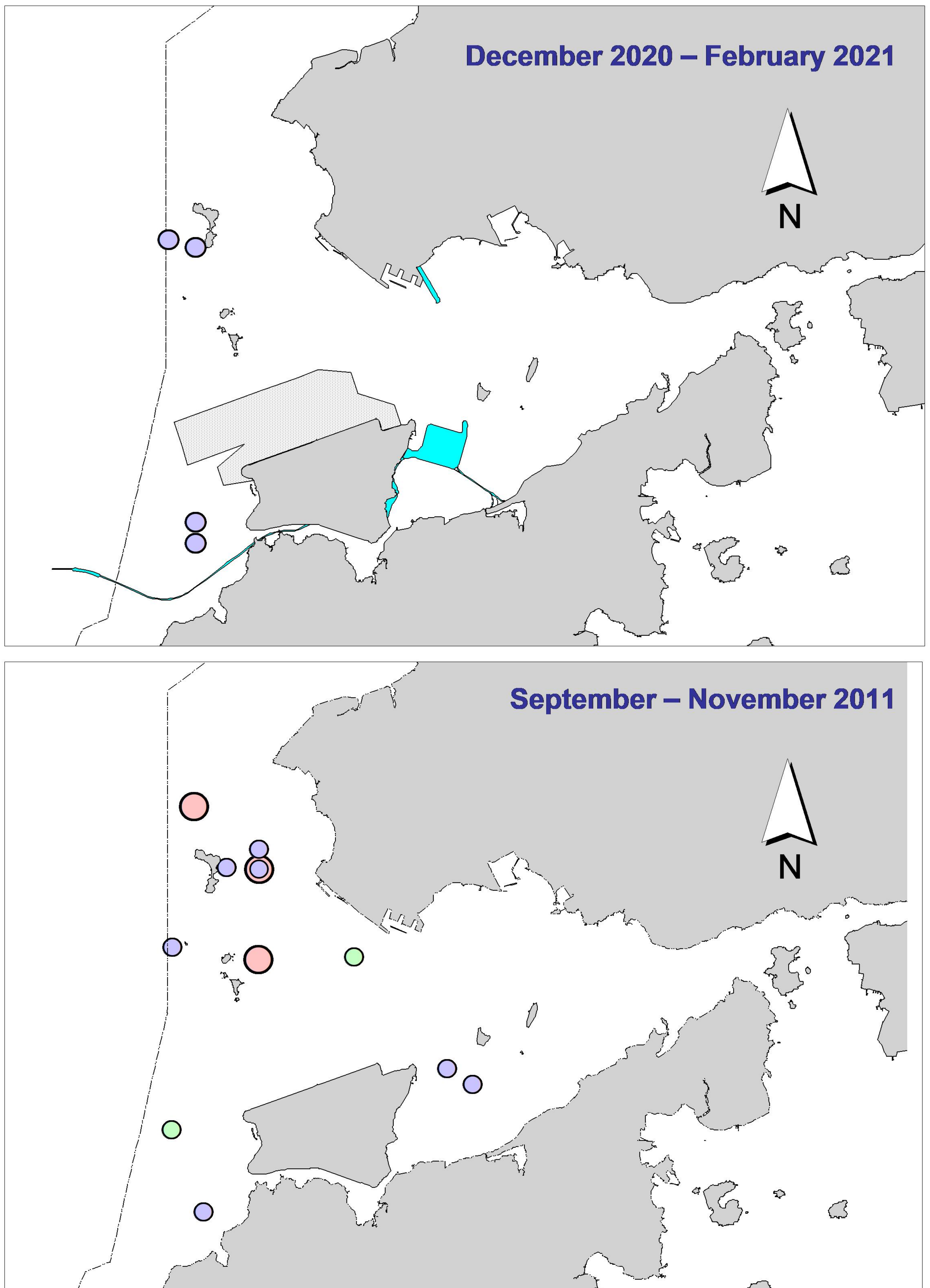
Figure 6. Distribution of Chinese white dolphins engaged in feeding (purple dots), socializing (pink dots) and traveling (green dots) activities during the present TMCLKL08 monitoring period (top) and baseline period in 2011 (bottom)
