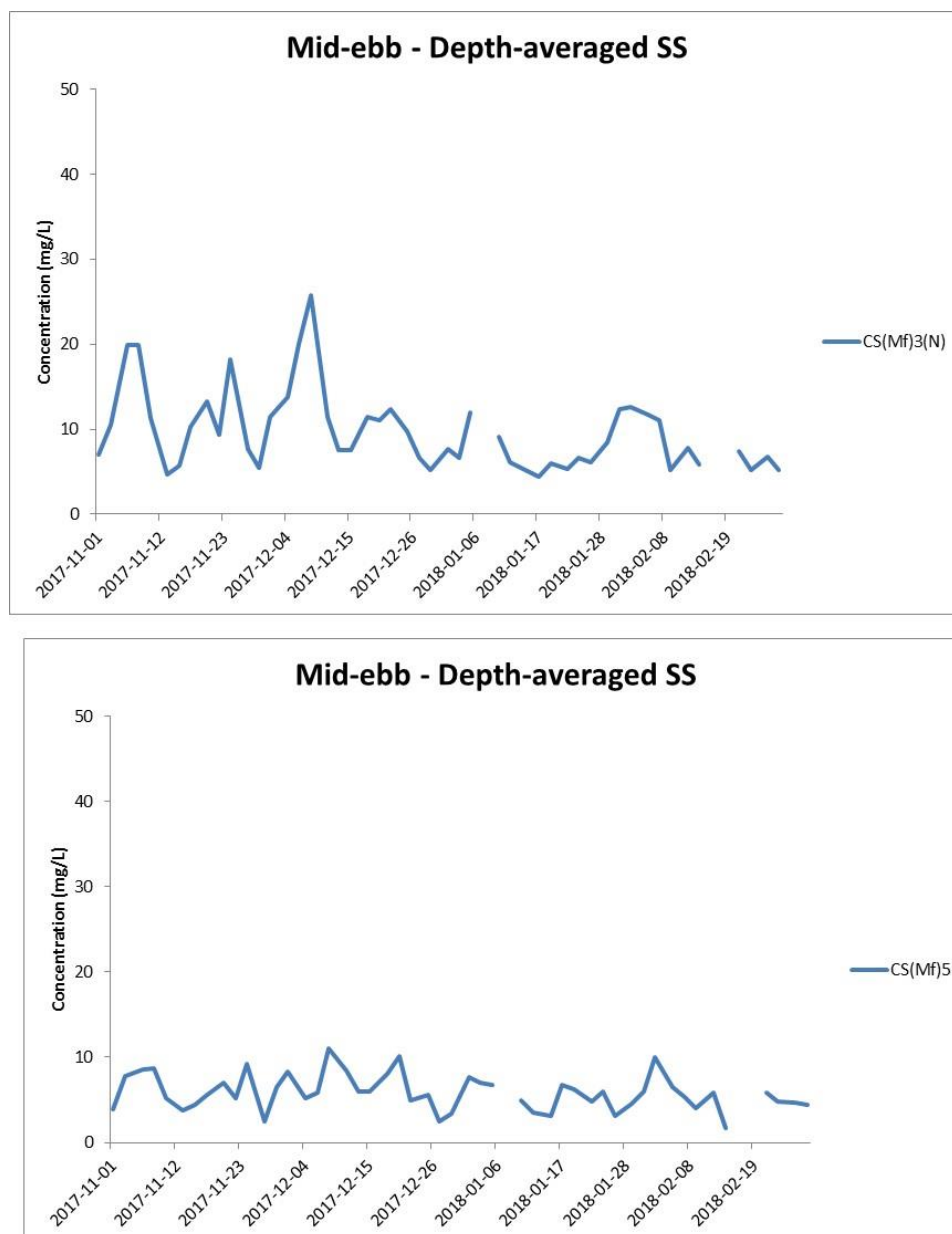
Figure J29 Impact Monitoring – Mean depth-averaged level of Suspended Solids (mg/L) during mid-ebb tide between 1 November 2017 and 28 February 2018 at CS(Mf)3(N) and CS(Mf)5.
