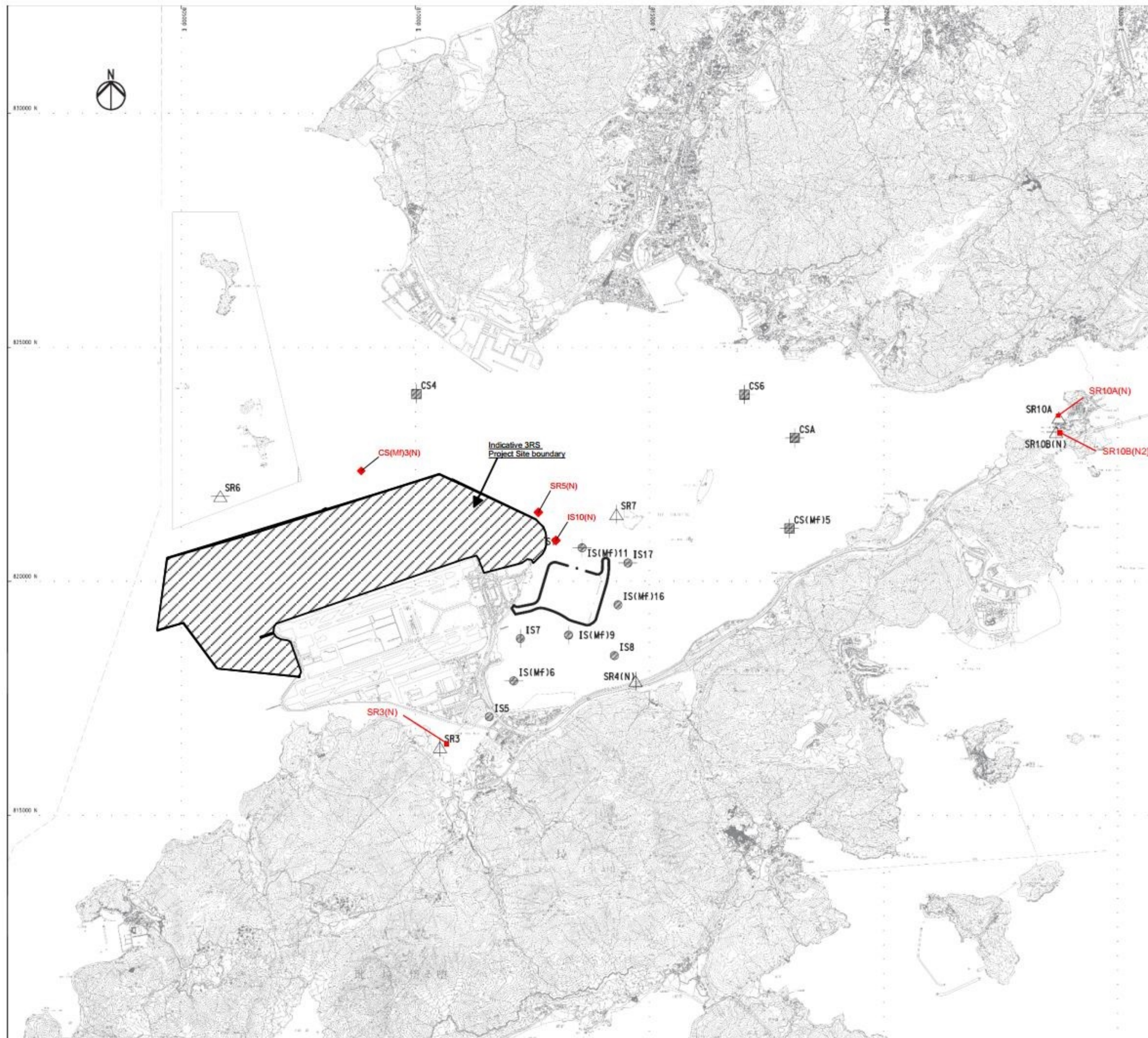
LEGEND IS IMPACT STATIONS CS CONTROL / FAR FIELD STATIONS SR SENSITIVE RECEIVERS STATIONS FIGURE 4.1— LOCATION OF WATER QUALITY MONITORING STATIONS SETTING OUT SCHEDULE
